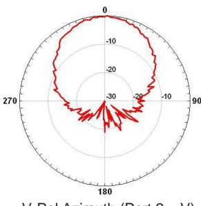
V-Pol Azimuth (Port 2 - V)
