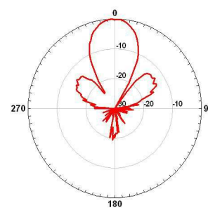
V- Pol Elevation (Port 1 - H)
