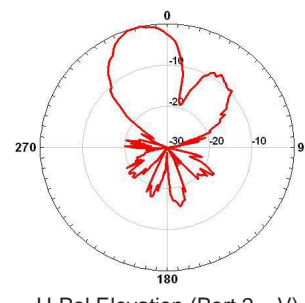
H-Pol Elevation (Port 2 - V)
