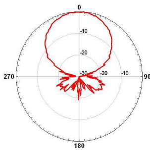
H-Pol Azimuth (Port 1 - H)
