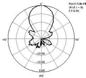
H-Pol Azimuth (Port 1 - H)
